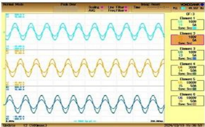
Figure 15. Waveforms of the voltage and current in the system with Grid Connected Mode
