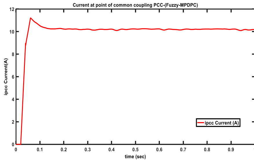
Figure 8. Current at PCC using Proposed method
