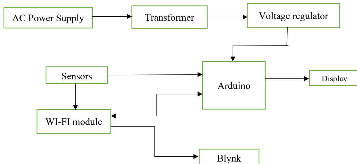
Fig 3: Block Diagram of the smart cradle using Blynk
