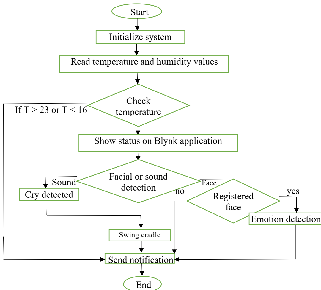
Fig 1: Flow chart of the proposed system
