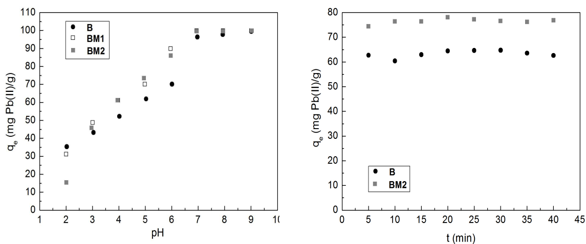
Figure 8 (left) Effect of pH of the solution on the Pb(II) adsorption
