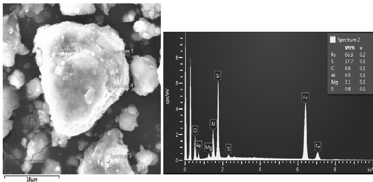
Figure 4 SEM image of composite material BM1 with EDX analysis
